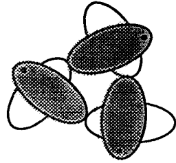
scFv-0 trimer
